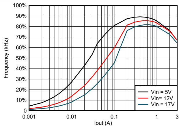
Figure 5-11. TPS563206 Efficiency at 0.6 Vout With 1.5uH Inductor
