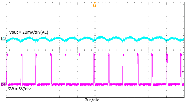
Figure 7-9. TPS563206 Output Voltage Ripple With 0.1A Loading
